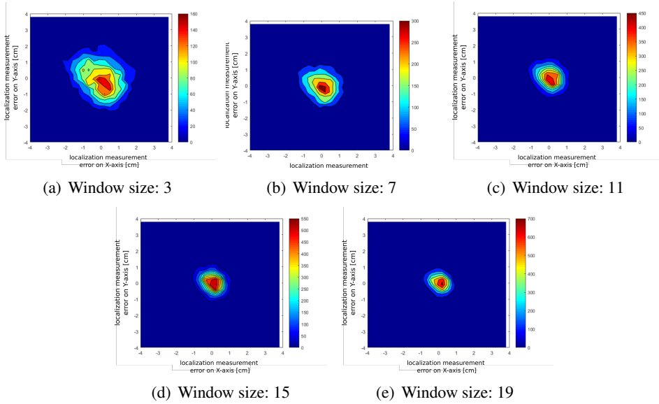
Figure 19: Median filter
