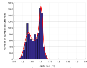
(d) Sample distribution disturbed by a human passing the direct route between the tag and the anchor
