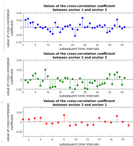
(b) The values of the cross-correlation coefficient between each pair of anchors
