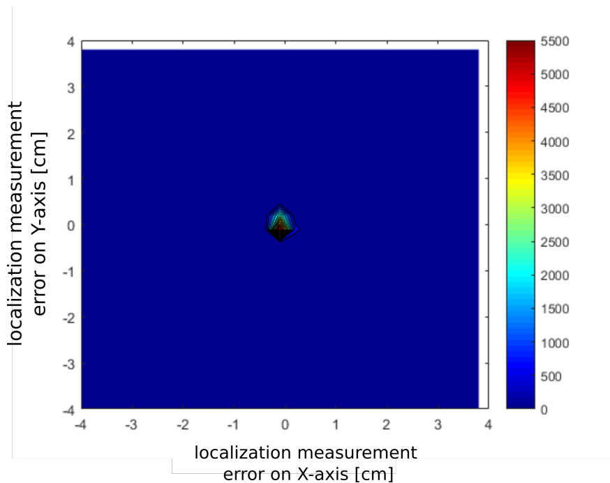
Figure 21: Distribution of sample positions in two-dimensional space at the location of a stationary object after using the Kalman filter
