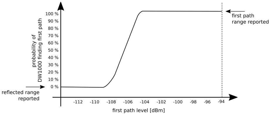
Figure 12: The graph of the probability that the DW1000 will find the first direct route depending on the signal level on this route [14]
