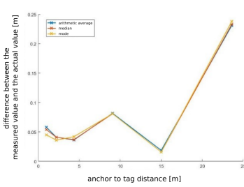
(a) The difference between the measured value and the actual value in relation to the distance of the tag from the anchor
