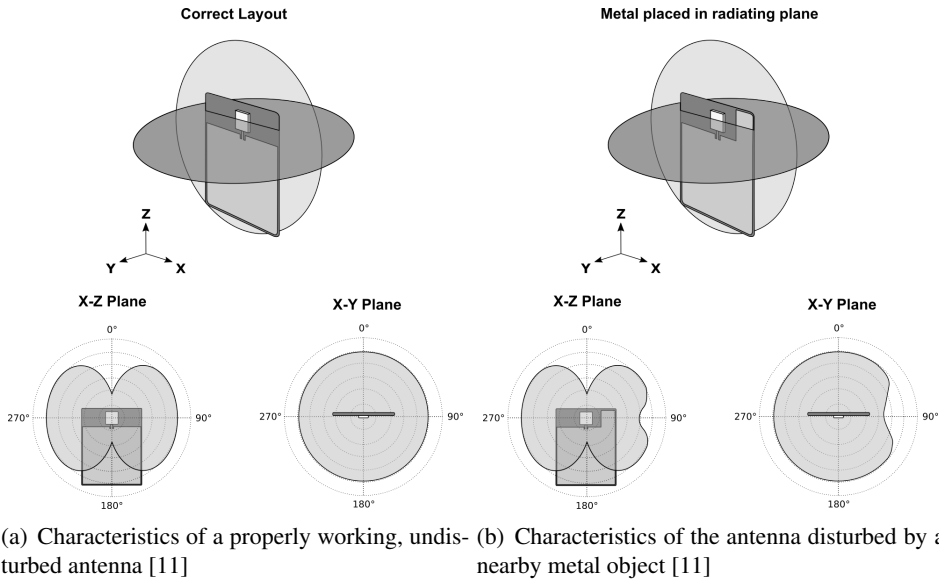
Figure 4: Antenna characteristics
