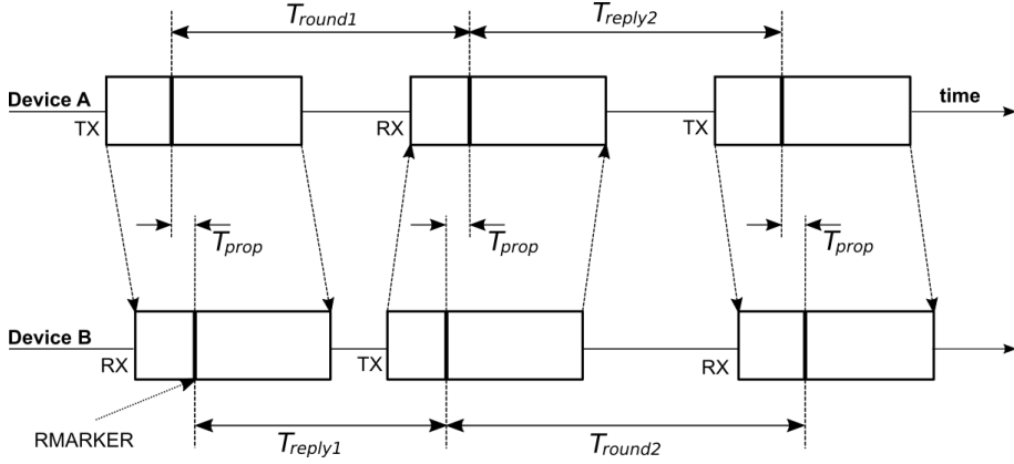
Figure 6: Scheme of message exchange between two devices [12]
