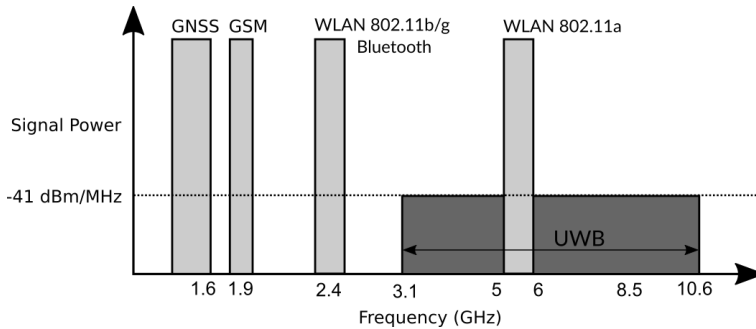
Figure 1: Comparison of popular technologies used for indoor locations in terms of used frequency and power spectral density. [1]
