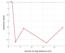
(b) The dependence of the variance value on the anchor distance from the tag
