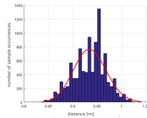
(g) Distance: 1.000m, Baud Rate: 110kbps, Average: 0.9356m, Standard Deviation: 0.0333.
