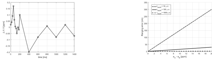
(a) Changes in the PPM value over time. The graph clearly shows the rapid changes in PPM in the first 400 ms of the oscillator operation, which is the result of its heating, as well as a natural physical phenomenon [13]
