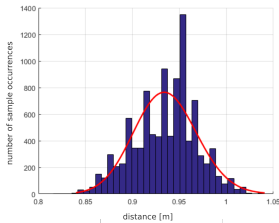
(a) Distance: 1.000m, Baud Rate: 110kbps, Average: 0.9356m, Standard Deviation: 0.0333.
