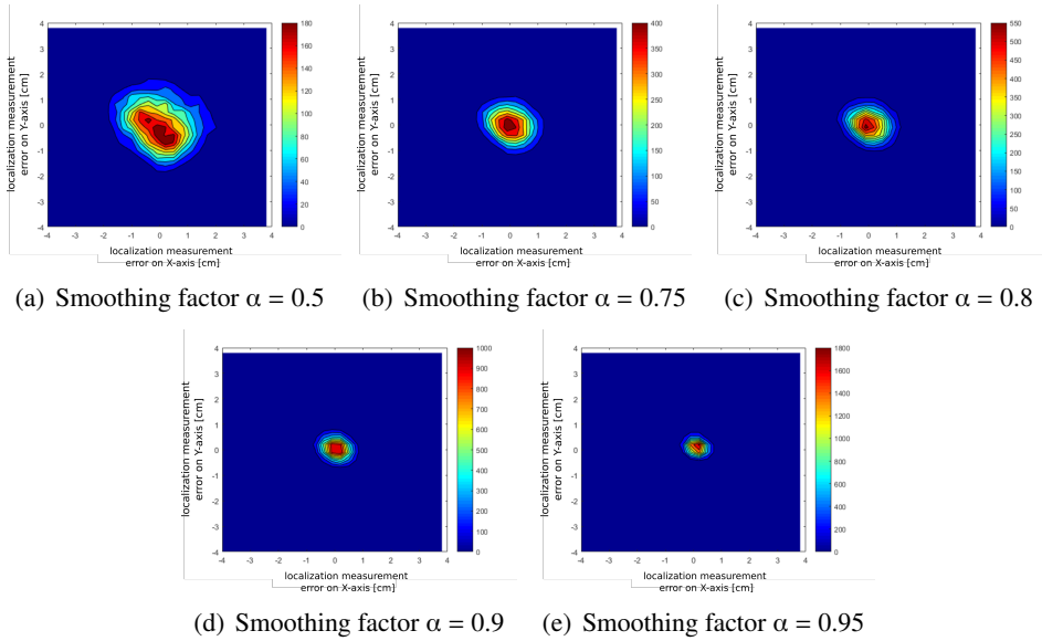
Figure 20: ARMA filter
