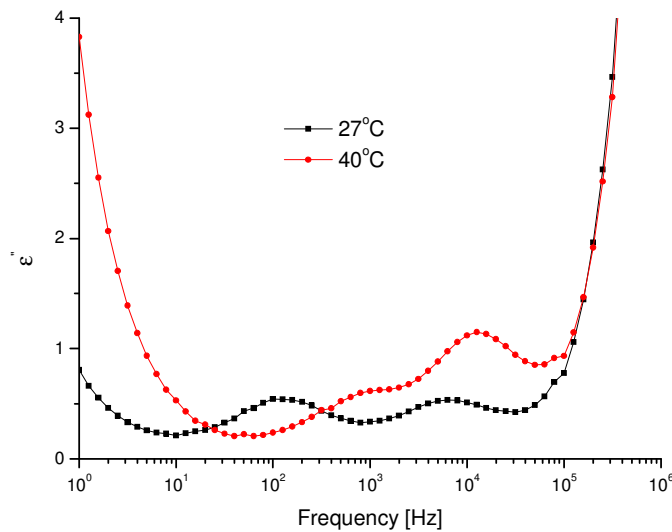
Fig. 2. Imaginary part of the dielectric spectrum of the M3No2 mixture at chosen temperatures as in Fig. 1, here two relaxation modes were registered in the ferroelectric phase in whole temperature range of phase existing
